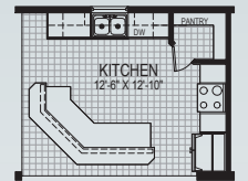
ALTERNATE 2 KITCHEN w/ LR06 ISLAND
